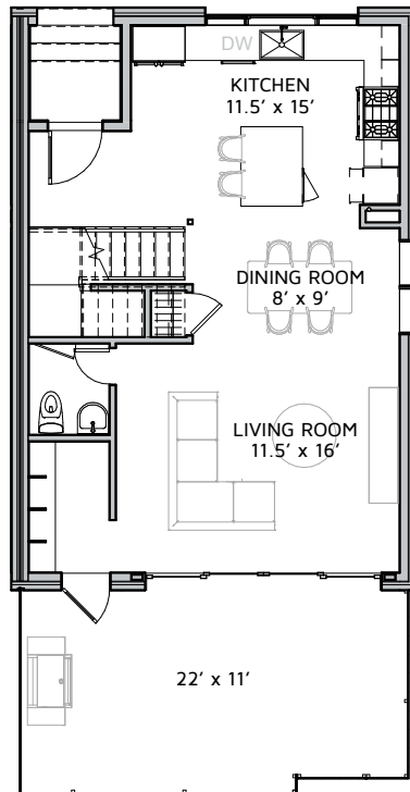
MAIN LEVEL
